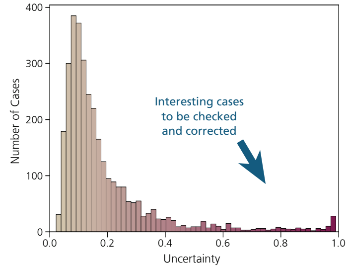
Uncertainty on 3200 MRIs (model trained with 100 cases)
